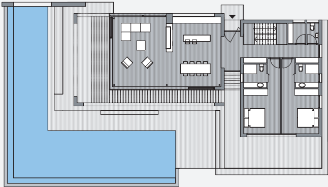
Grundriss EG / ground level
