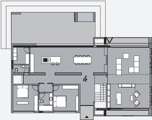
Grundriss EG / ground level
