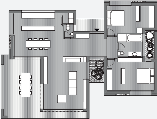
Grundriss / ground plan
