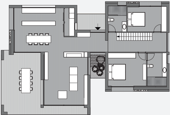
Grundriss EG / ground level
